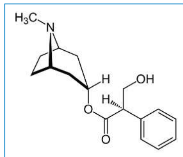
Figure 3 Atropine.
