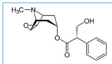
Figure 4 L-scopolamine.
